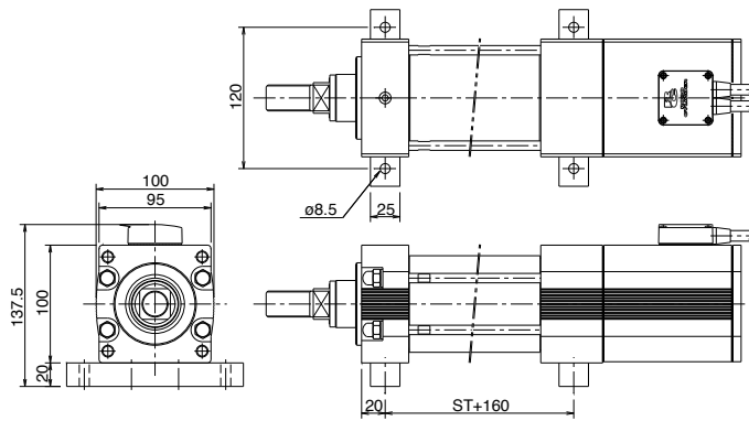
Foot Bracket (Code: FT)
