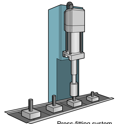
Press-fitting system
