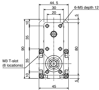
Guide installation direction (View A)
